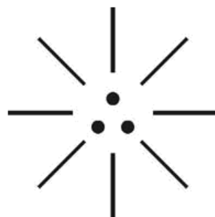
(Neutrino Radiation)
