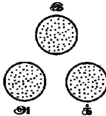
(CNO Species)
