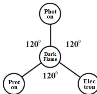
(Neutrino Oscillation)
