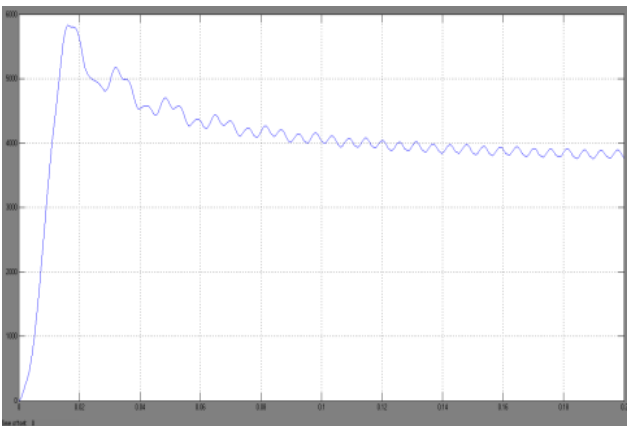
Fig.13 DC capacitor voltage ( V_{dc} ), KV
