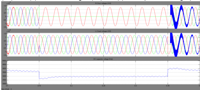
Fig.15 System response during L-L-G fault at bus B-2: (a) B-2 bus voltages ( V_{12} ), KV, (b) L-2 load voltages ( V_{12} ), KV, (c) DC capacitor voltage ( V_{dc} ),KV. The above waveforms shows when a 10 cycle L-L-G fault occurs at 0.15s such that both the a and b-phases of B-2 bus voltage become zero. B-2 bus voltages are shown in Fig.15 (a). It can be seen from Fig.15 (b) that the L-2 load voltages remain balanced.
