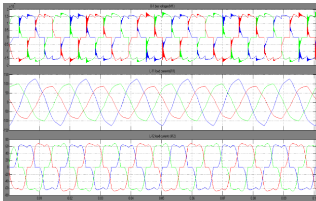
Fig.5 Simulation results – in absence of IUPQC: a) B-1 bus voltages ( V_{11} ),KV, (b) L-11 load currents ( i_{11} ),A and (c) L-12 load currents ( i_{12} ),A.
