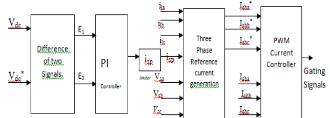
Fig .8 Block diagram for generation of gating signals
