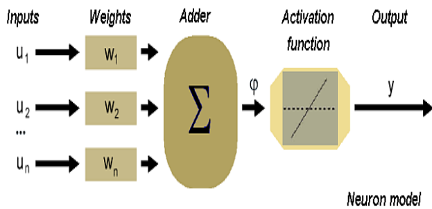
Figure 2. Neuron Model
