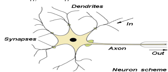
Figure1. Neuron Scheme
