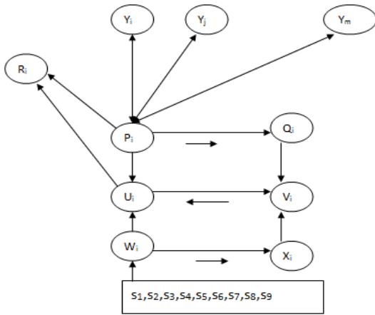
Figure3. ART2 architecture
